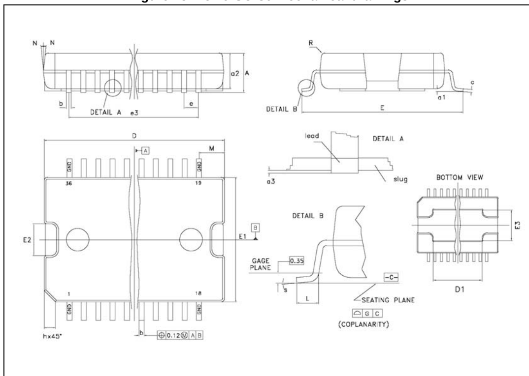
Figure 23. PowerSO-36 mechanical drawings
