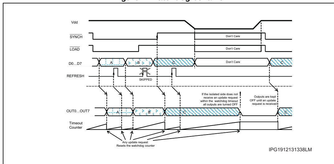
Figure 7. Watchdog behavior
