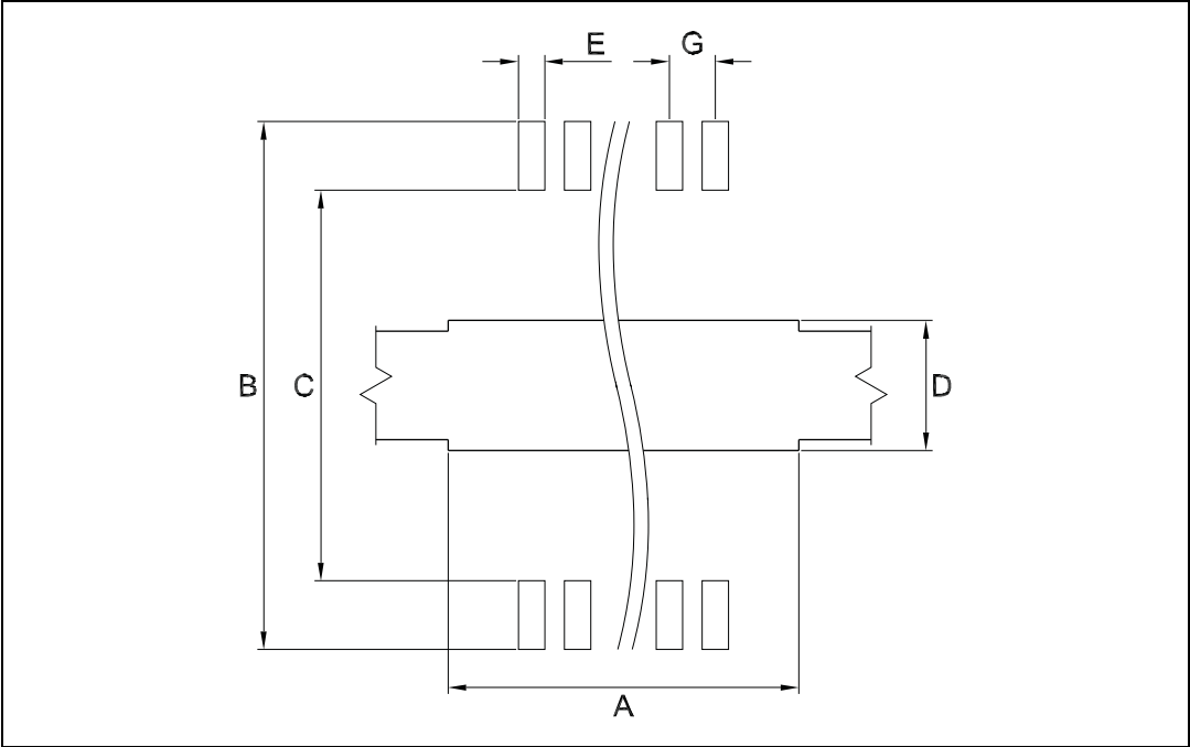
Figure 24. Footprint recommended data
