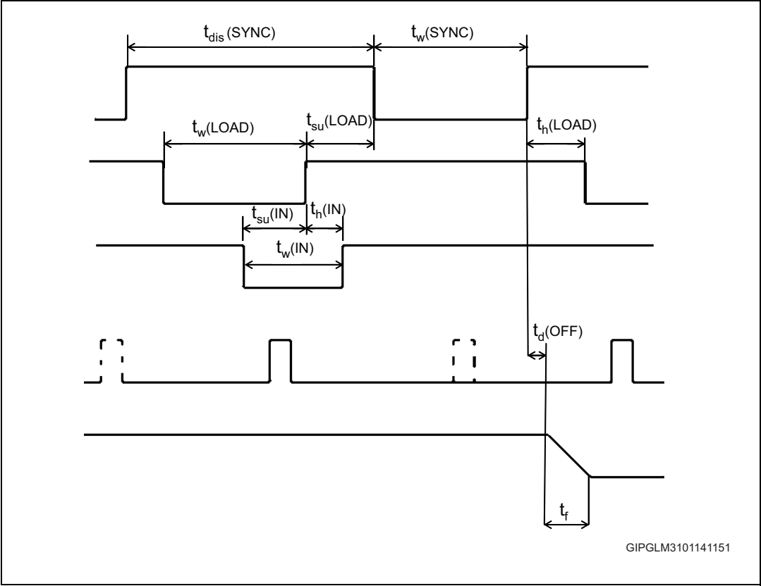
Figure 13. Multiple device synchronous control mode
