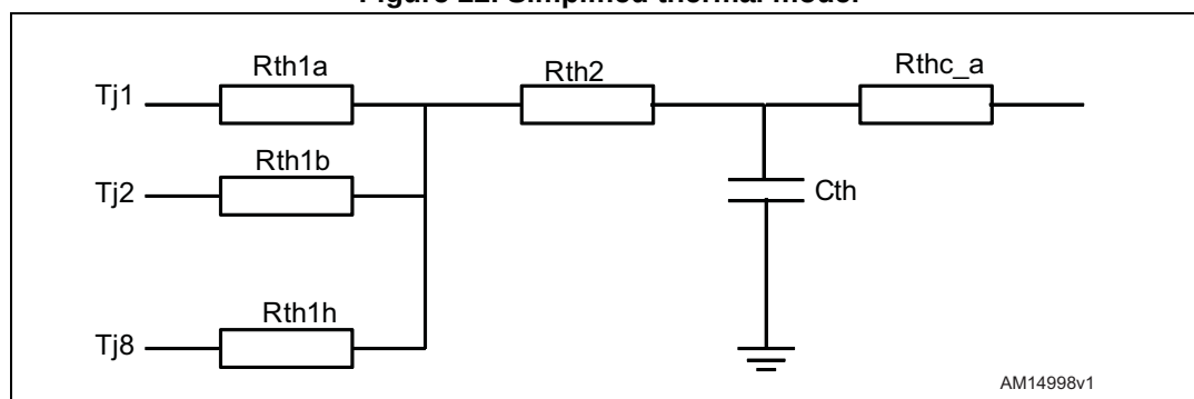
Figure 22. Simplified thermal model
