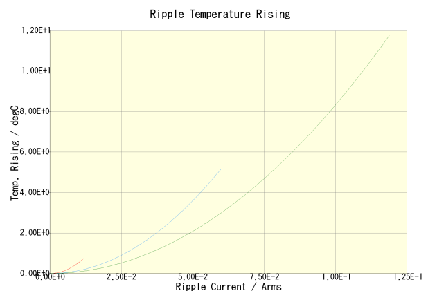
CKCA43X7R1H102M100AA(100kHz) CKCA43X7R1H102M100AA(500kHz) CKCA43X7R1H102M100AA(1MHz)
