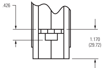
Captive Nut (-F1)
