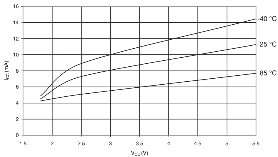
Figure 26-137. Programming Current vs. V_{CC}
