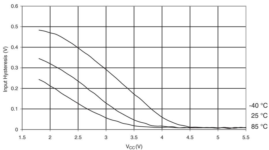
Figure 26-124. Reset Pin Input Hysteresis vs. V_{CC}
