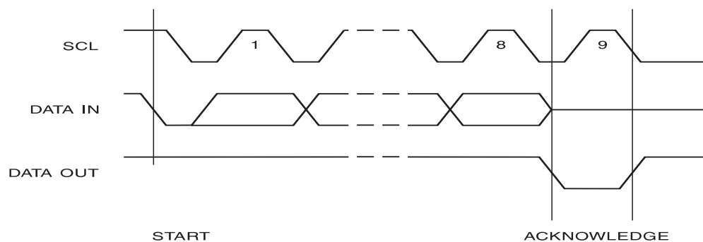
Figure 6. Output Acknowledge
