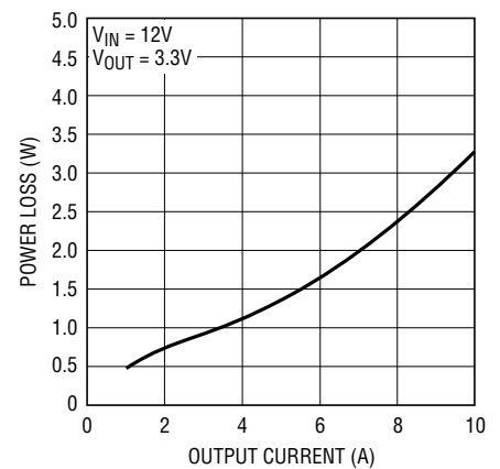
Figure 13. Power Loss vs Load Current
