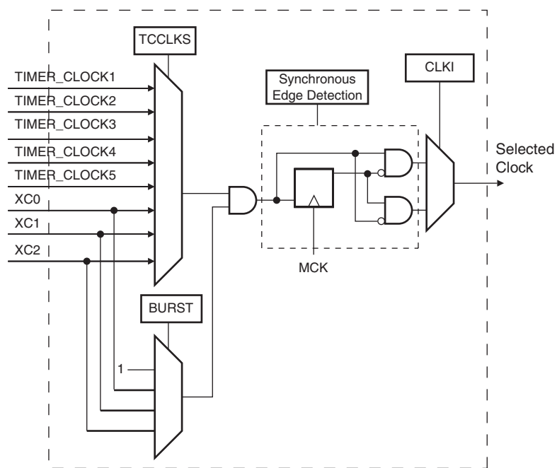
Figure 31-3. Clock Selection
