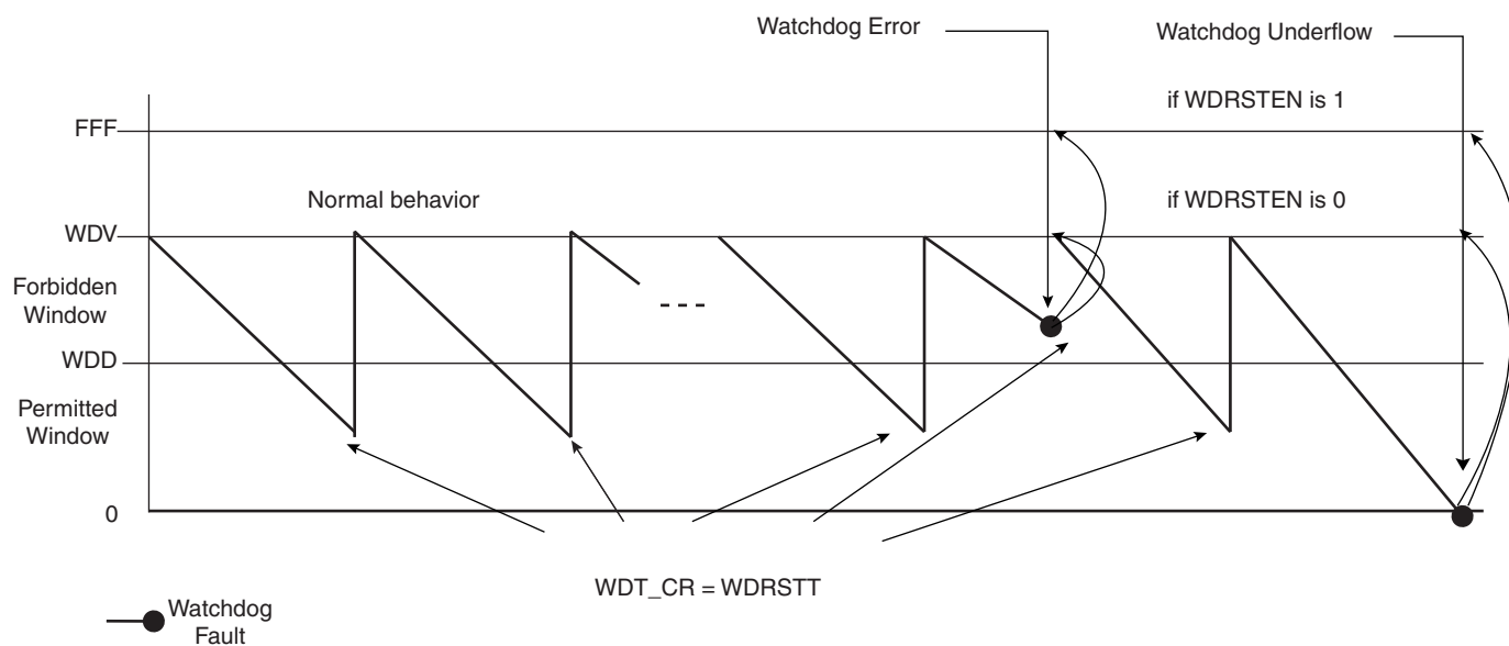
Figure 15-2. Watchdog Behavior
