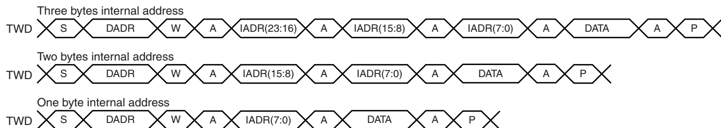
Figure 28-11. Master Write with One, Two or Three Bytes Internal Address and One Data Byte
