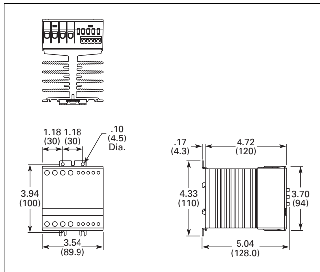
Figure 39-4. 90 mm Frame — Approximate Dimensions in Inches (mm)
