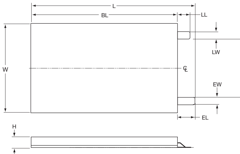
Case Dimensions: mm (inches) Case Size L ±0.5 (0.020) W +1.0 (0.040)/-0 H (Maximum) B ±0.5 (0.020) LL ±0.2 (0.008) LW ±0.2 (0.008) EL ±0.5 (0.020) EW ±0.5 (0.020) BZ01 30.5 (1.201) 17 (0.669) See Section 1 11.2 (0.441) 2.5 (0.098) 1.4 (0.055) 2.5 (0.098) 1.4 (0.055) BZ05 23.5 (0.925) 15 (0.591) See Section 1 7.5 (0.295) 2.5 (0.098) 2.5 (0.098) 3.5 (0.138) 2.5 (0.098) BZ09 20.5 (0.807) 15 ( 0.591) See Section 1 7.5 (0.295) 2.5 (0.098) 2.5 (0.098) 3.5 (0.138) 2.5 (0.098)
