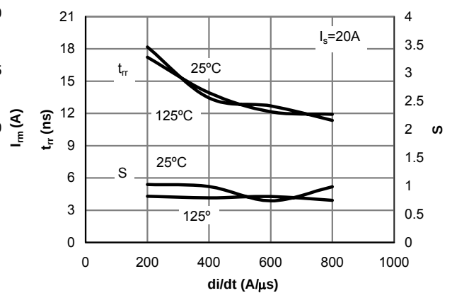
Figure 21: Diode Reverse Recovery Time and Softness Factor vs. di/dt
