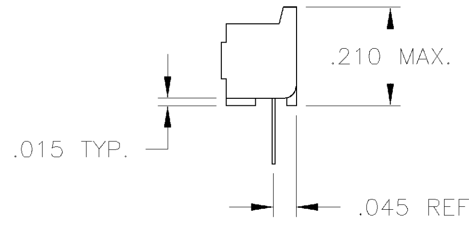
SECTION A-A ROTATED 90° CW SCALE 10:1 FOR -6,-7 & -8 ONLY
