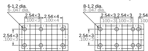
PC board pattern (Copper-side view)
