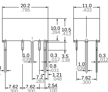
2 coil latching
