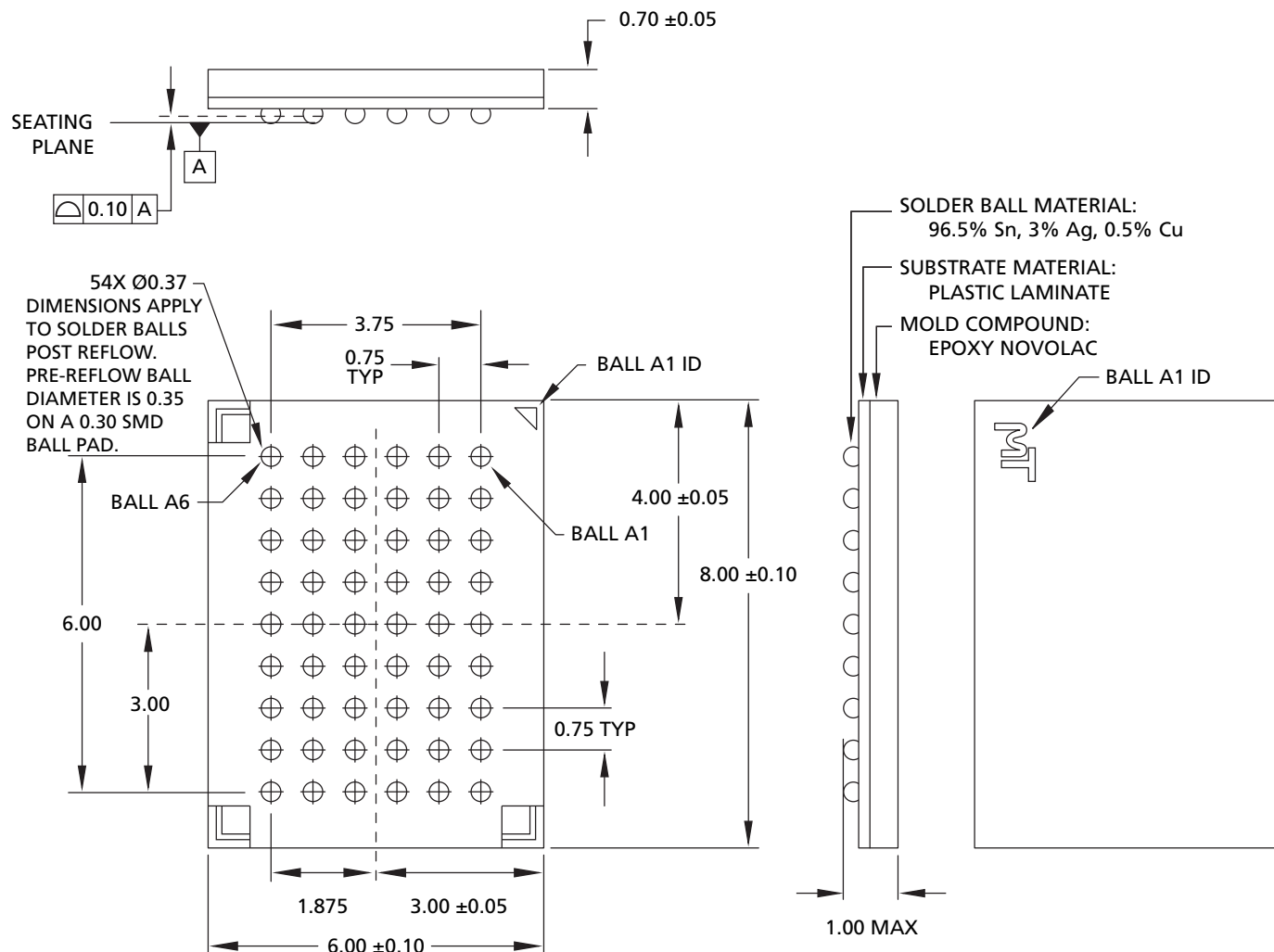
Figure 47: 54-Ball VFBGA
