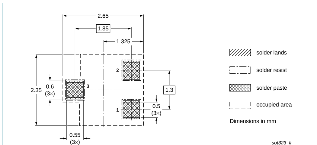
Fig 20. Reflow soldering footprint PDTC114EU (SOT323/SC-70)
