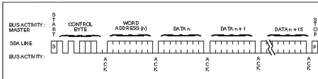
FIGURE 8-1: PAGE WRITE
