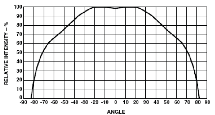
Figure 4 Radiation Pattern
