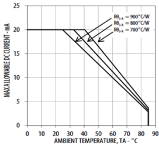
Figure 5 Derating Curve
