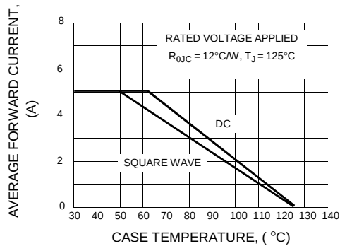
FIG.1 - CURRENT DERATING (CASE)
