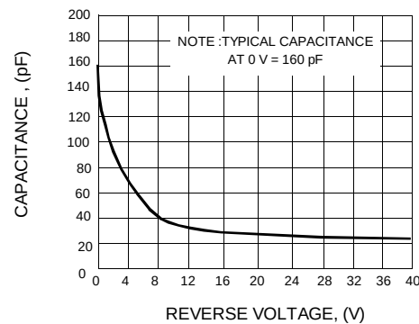
FIG. 5 TYPICAL CAPACITANCE
