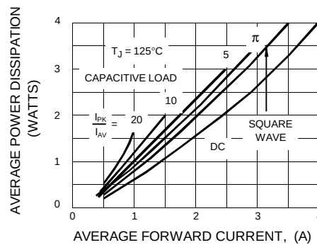
FIG.2 - POWER DISSIPATION
