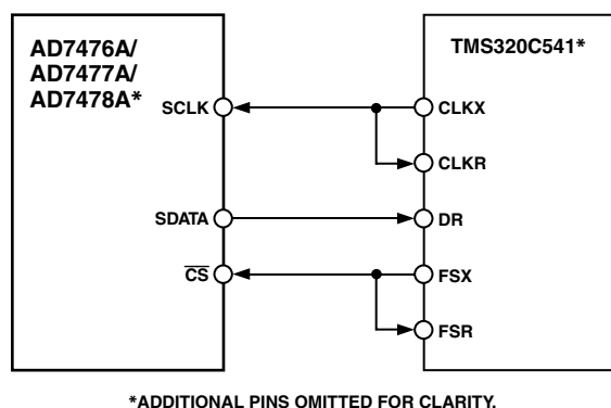
Figure 17. Interfacing to the TMS320C541
