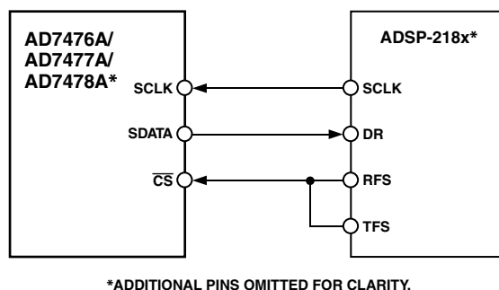
Figure 18. Interfacing to the ADSP-218x
