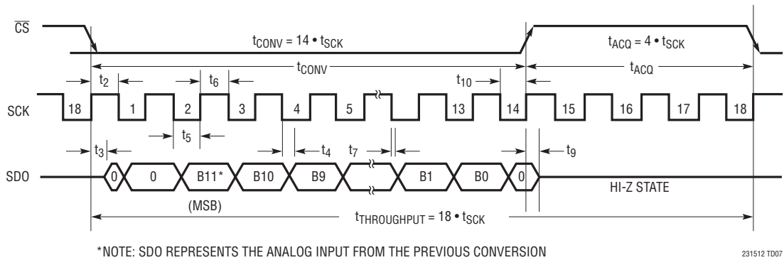
Figure 7: LTC2315-12 Serial Interface Timing Diagram (SCK Continuous)
