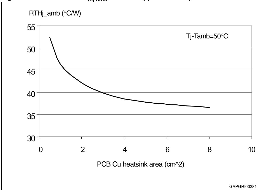
Figure 36. PowerSO-10 R_{thj-amb} vs PCB copper area in open box free air conditions
