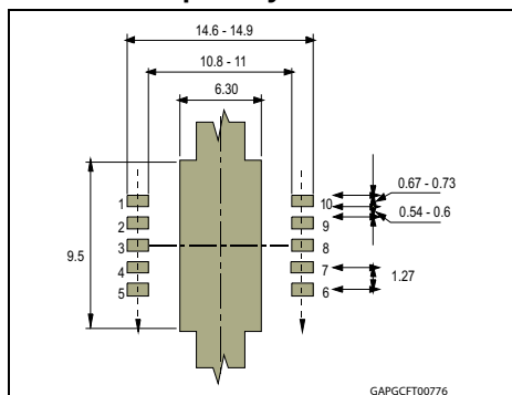
Figure 49. PowerSO-1 pad layout
