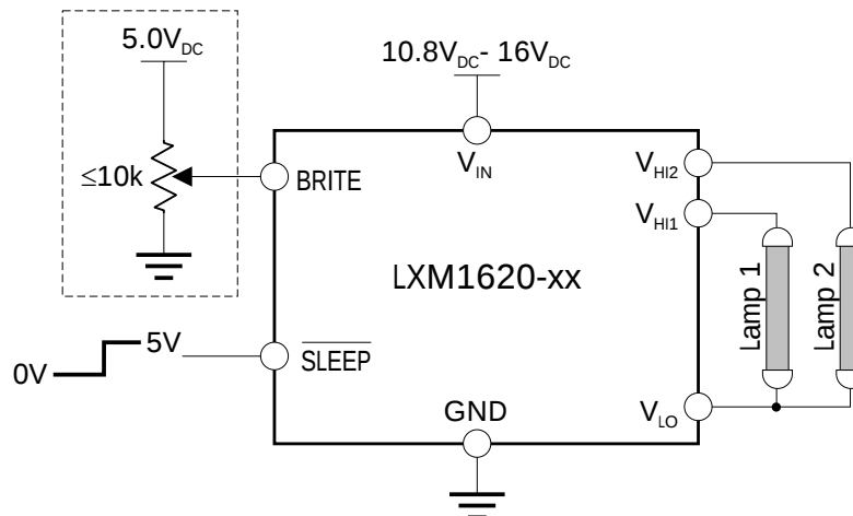
FIGURE 4 — Potentiometer Brightness Control
