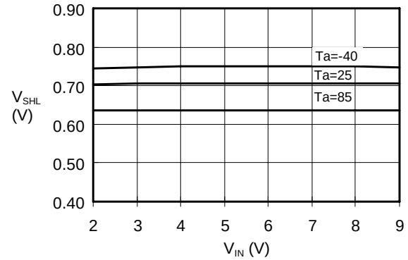
V_{SHL} - V_{IN} S-8330A/B/31A
