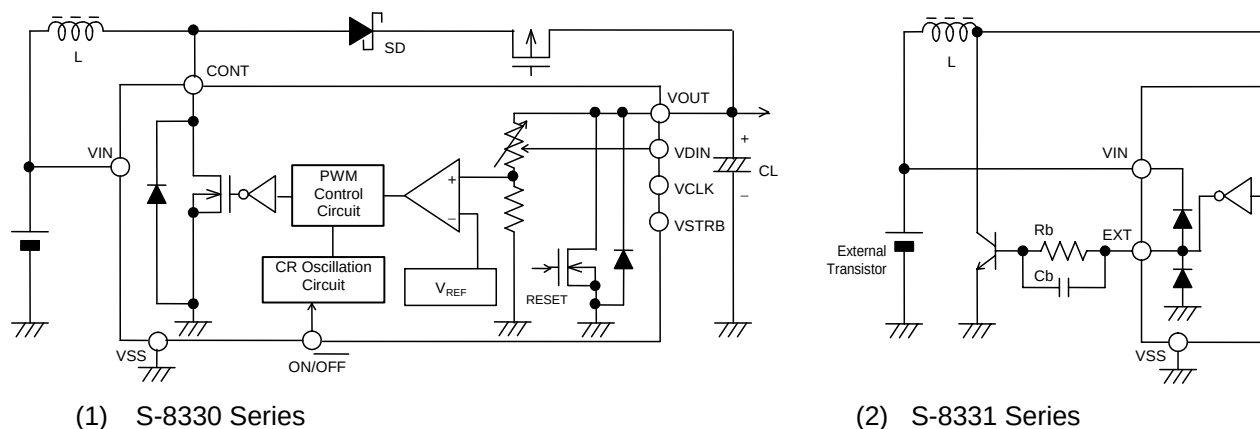
Figure 1 Block Diagram
