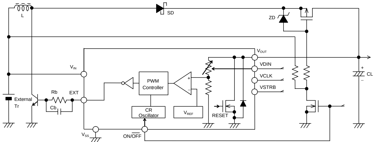
Figure 15 S-8330 Series
