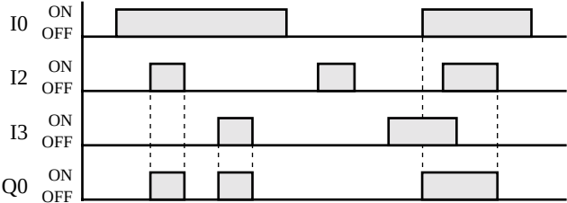
Timing Chart
