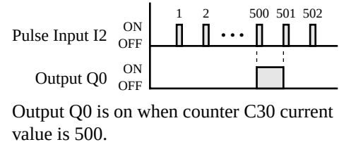
Timing Chart
