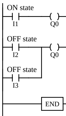
Ladder Diagram
