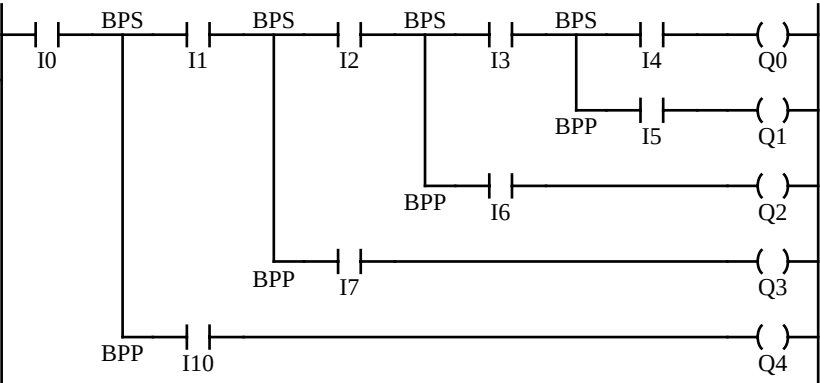
Ladder Diagram
