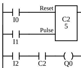
Ladder Diagram (CNT2 to 31)
