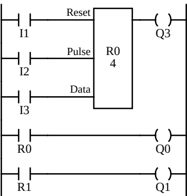
Ladder Diagram
