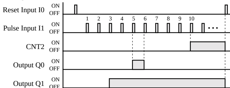
Timing Chart
