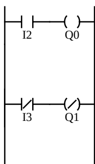
Ladder Diagram
