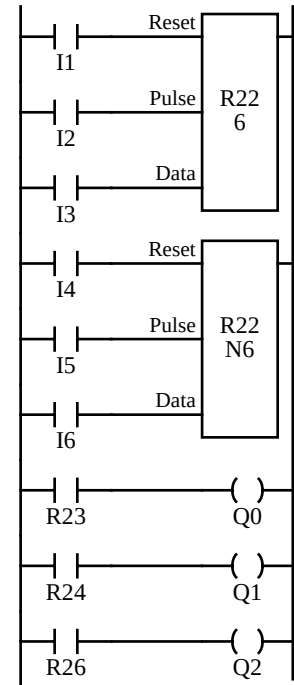
Ladder Diagram
