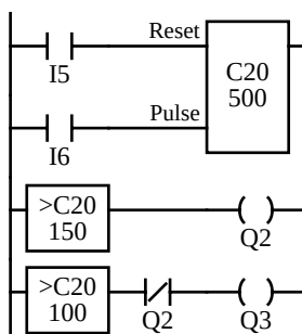
Ladder Diagram 4
