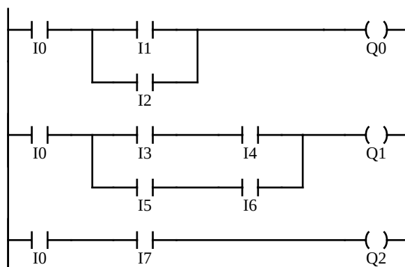
Ladder Diagram
