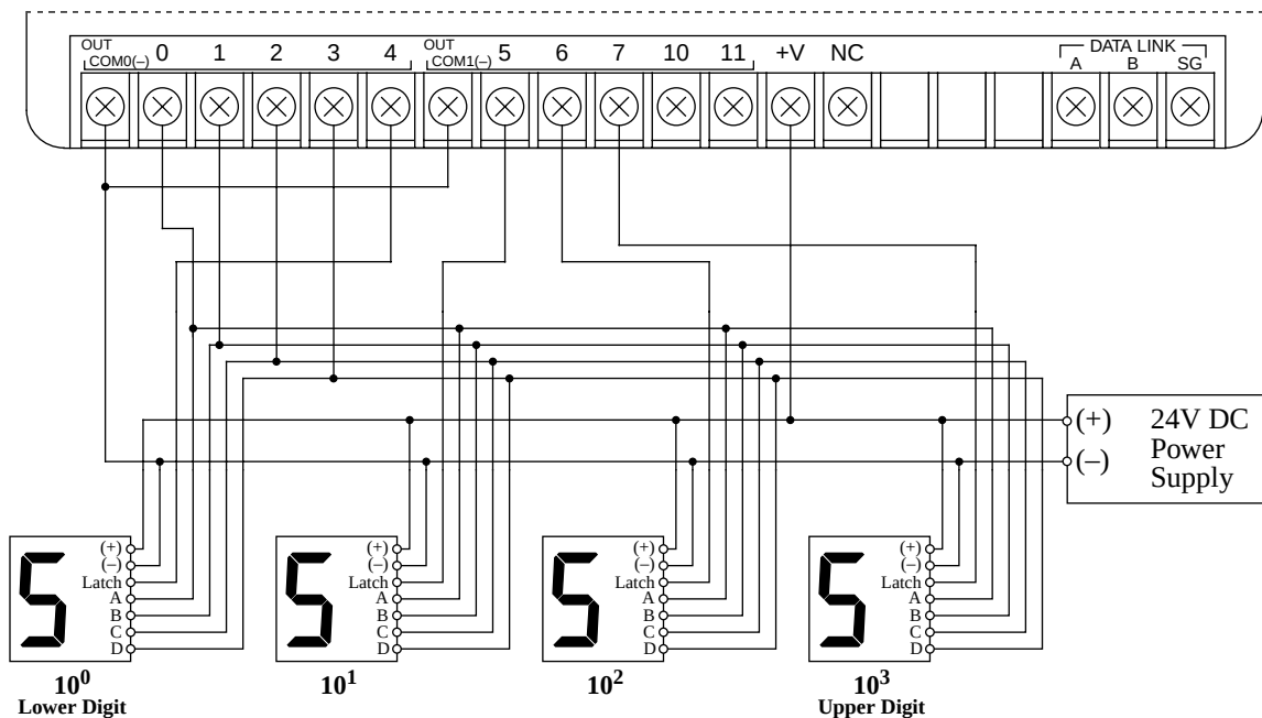
MICRO 3 Base Unit FC2A-C24B1 (Transistor Sink Output)
