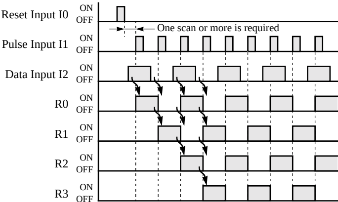
Timing Chart
