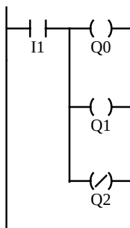
Ladder Diagram
