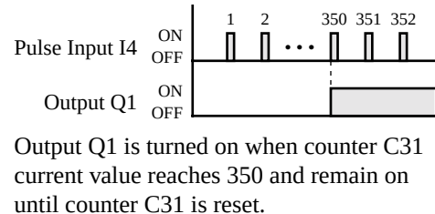
Timing Chart
