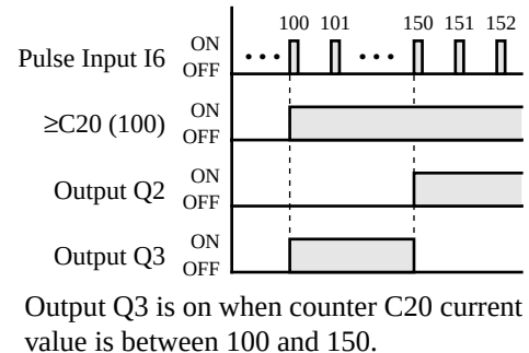
Timing Chart
