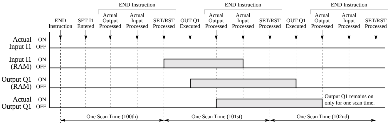
Time Chart for SET and RST Operation
