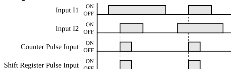
Timing Chart
