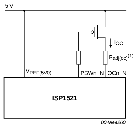
Fig 18. Adjusting analog overcurrent detection limit (optional)
