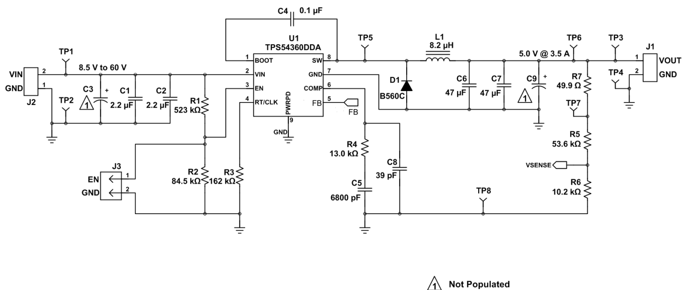
Figure 27. TPS54360EVM-182 Schematic
