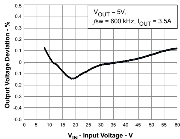
Figure 6. Regulation Versus Input Voltage
