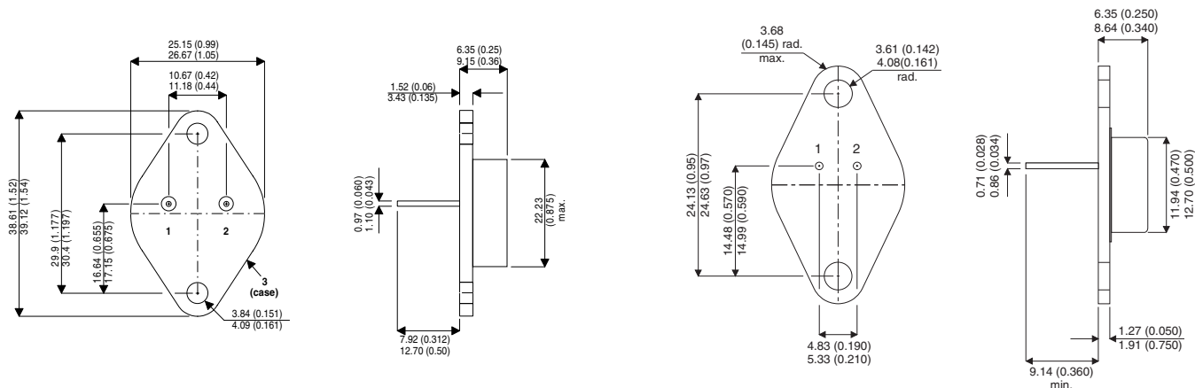
K-Package (TO-3)
