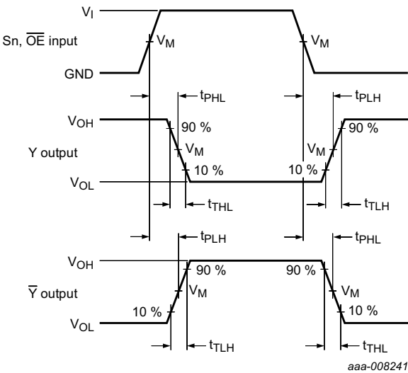
Measurement points are given in Table 8 . V_{OL} and V_{OH} are typical voltage output levels that occur with the output load. Fig 7. Propagation delay input (Sn, \overline{OE} ) to output (Y, \bar{Y} )
