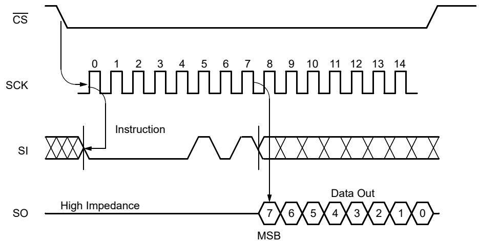
Figure 6. Read Status Register Sequence
