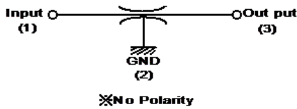
a)Equivalent Circuit
