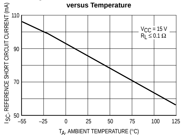
Figure 8. Reference Short Circuit Current versus Temperature
