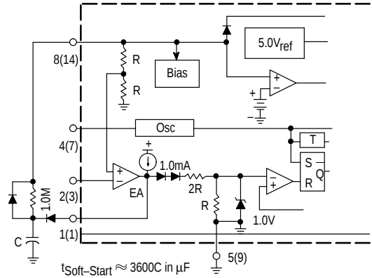
Figure 20. Soft-Start Circuit
