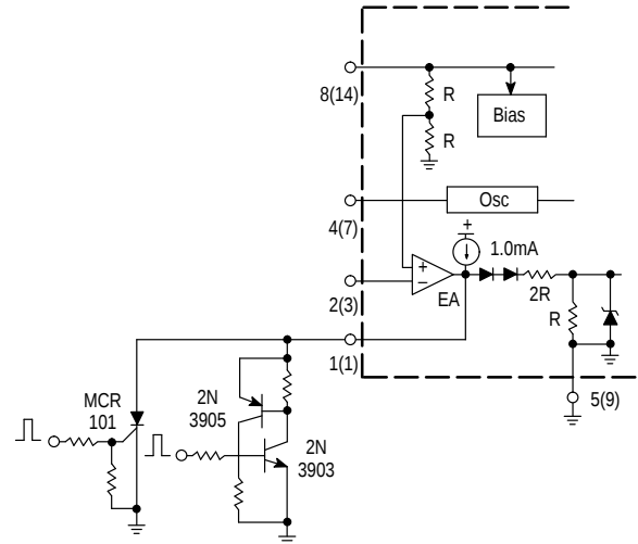
Figure 27. Latched Shutdown
