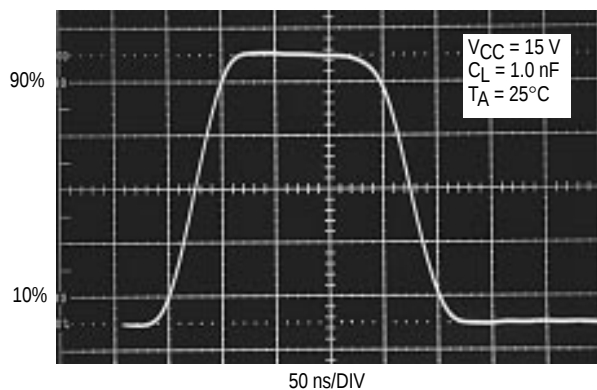
Figure 12. Output Waveform
