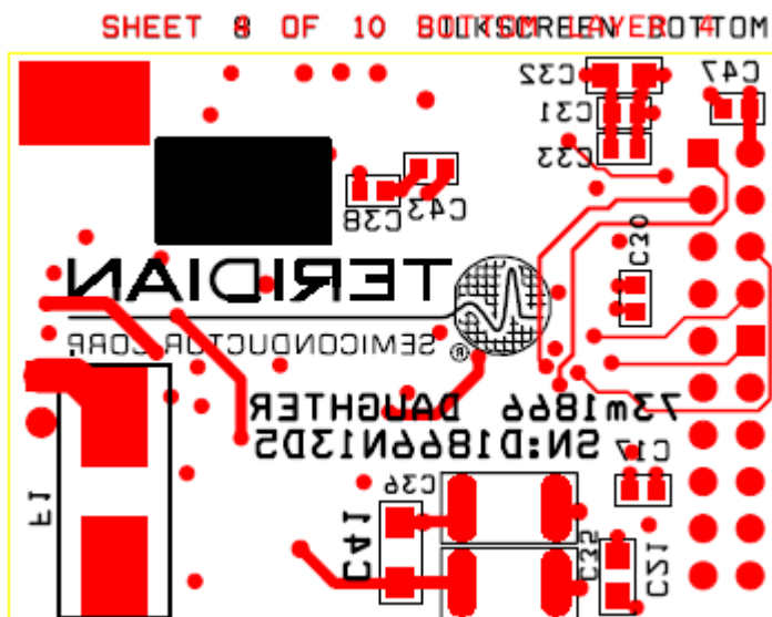
Figure 4: 73M1866B Keychain Demo Board Bottom Layer
