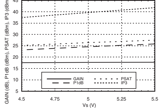
Gain, Power & Output IP3 vs. Supply Voltage @ 900 MHz
