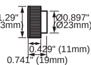
OCW-11 Pushbutton Rubber Boot
