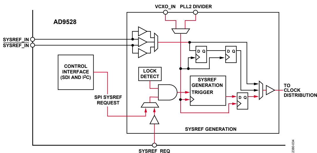
Figure 39. Mode 3, SYSREF Generated Internally and Routd to the Clock Distribution
