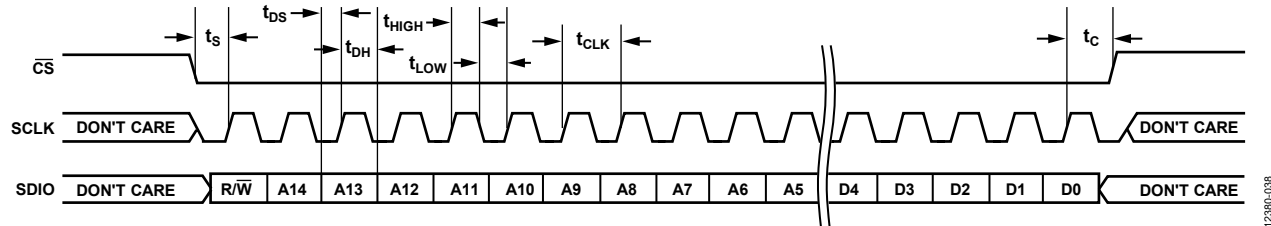
Figure 42. Timing Diagram for Serial Control Port Write—MSB First
