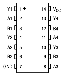
Figure 2. PIN ASSIGNMENT
