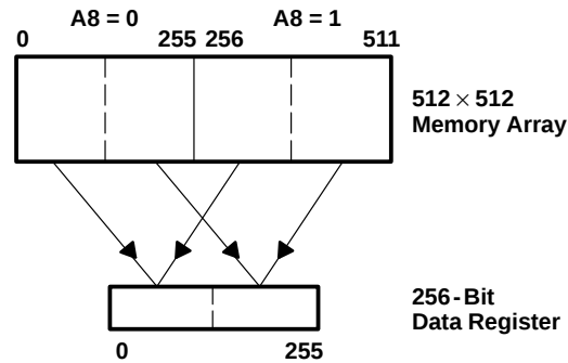
Figure 21. Split-Register-Transfer Read
