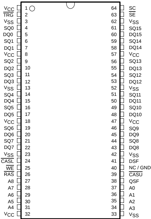
DGH PACKAGE (TOP VIEW)
