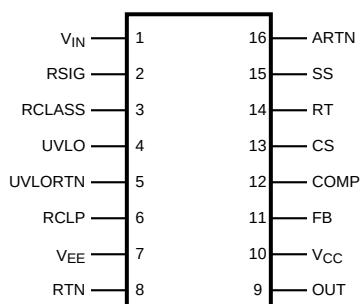
Figure 2. 16 Lead TSSOP/WSO See Package Number PW or NHQ0016A
