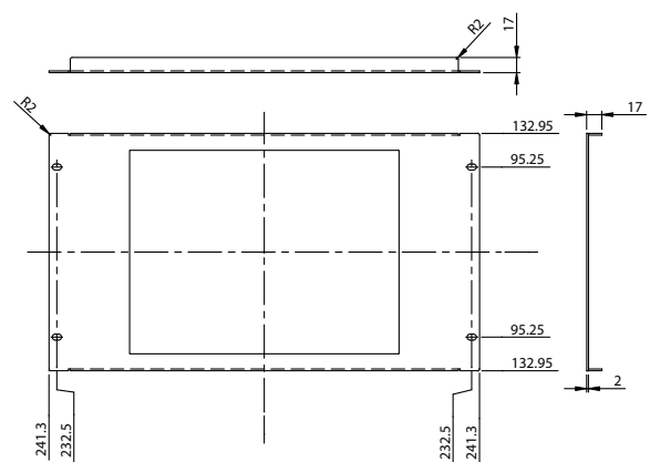
19" Rack plate (6U) for PPC-S123
