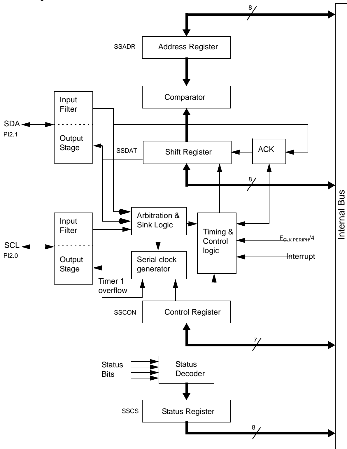
Figure 50. Block Diagram
