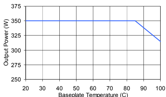
Figure 20. Output Power Derating for JNC350R in Conduction cooling (cold plate) applications; T_a < 70^\circ\text{C} in vicinity of module interior; V_{IN} = 24V .
