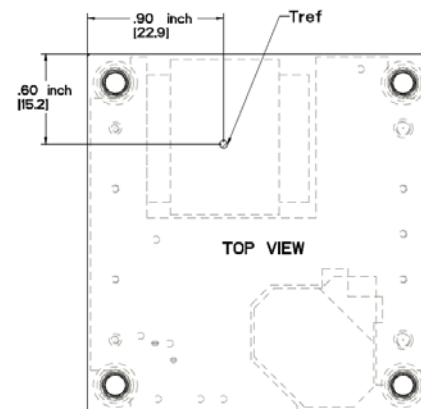
Figure 19. Case ( T_{REF} ) Temperature Measurement Location (top view).
