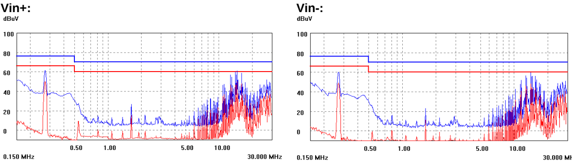
Figure 21. EMC considerations.
