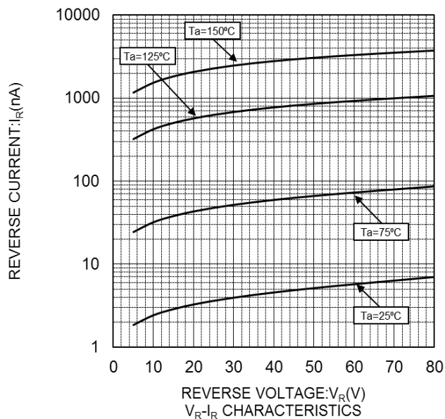
Fig.1 Reverse Current vs. Reverse Voltage
