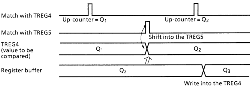
Figure 3.9 (12). Operation of Register Buffer
