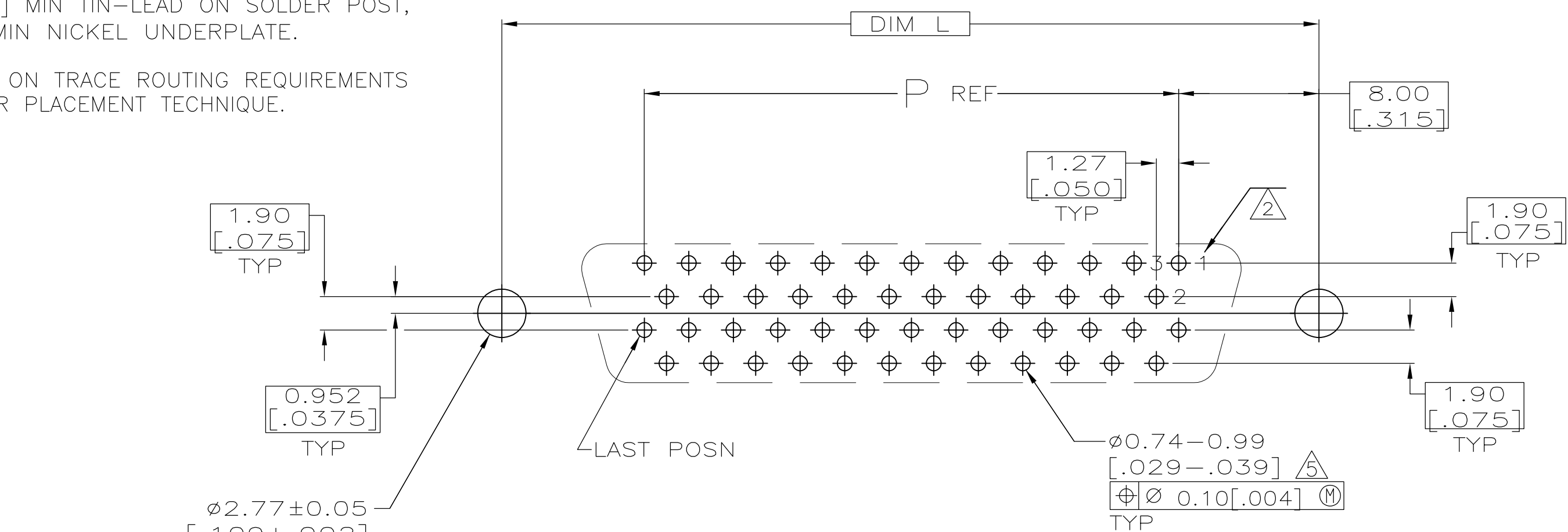
DETAIL Y CONNECTOR SIDE OF BOARD
