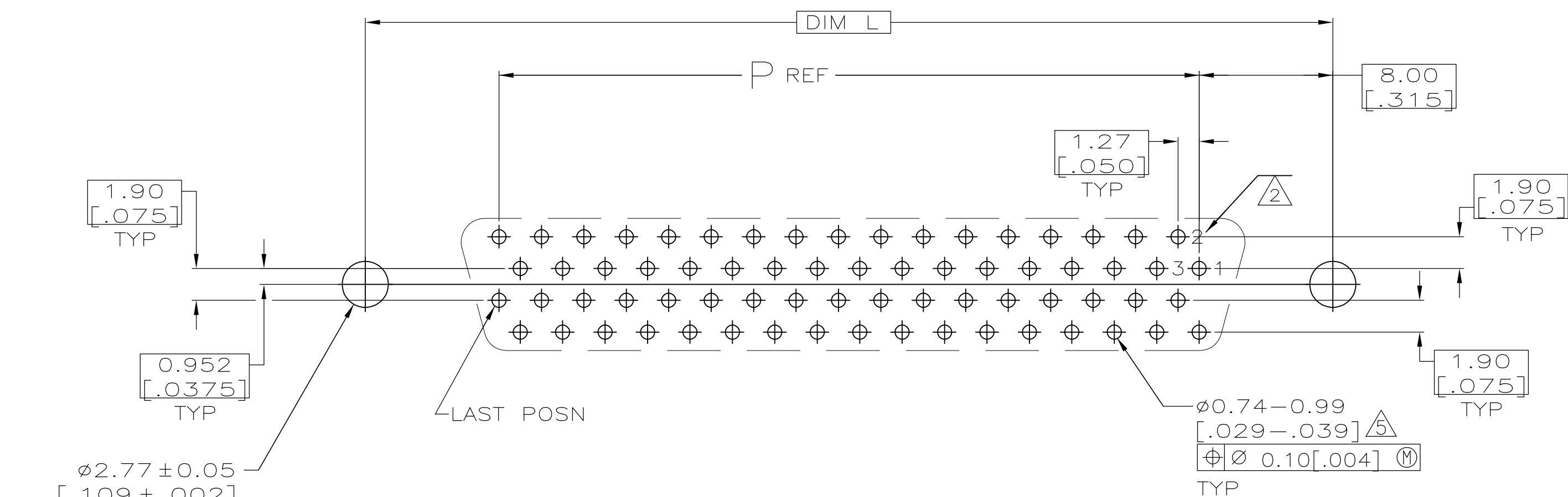
DETAIL X CONNECTOR SIDE OF BOARD
