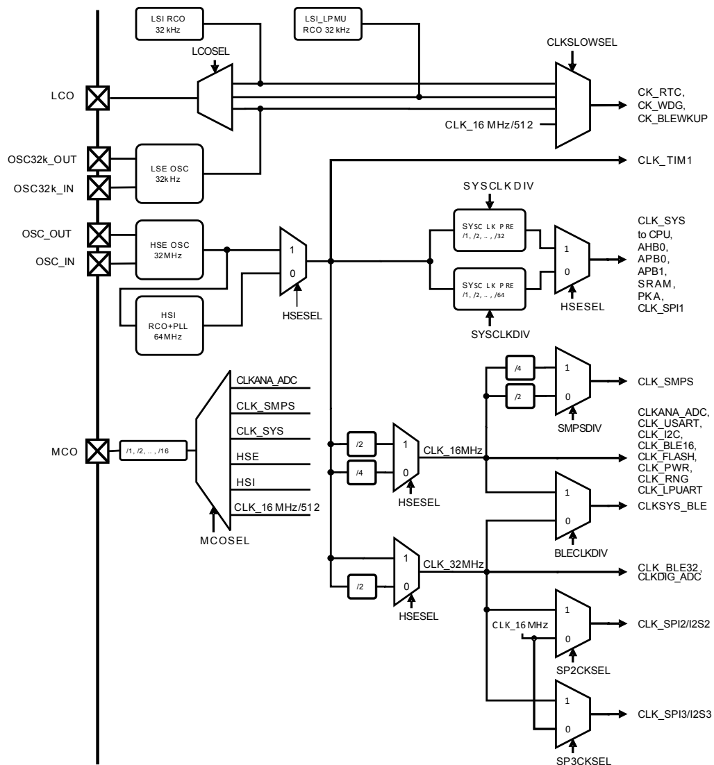
Figure 6. Clock tree
