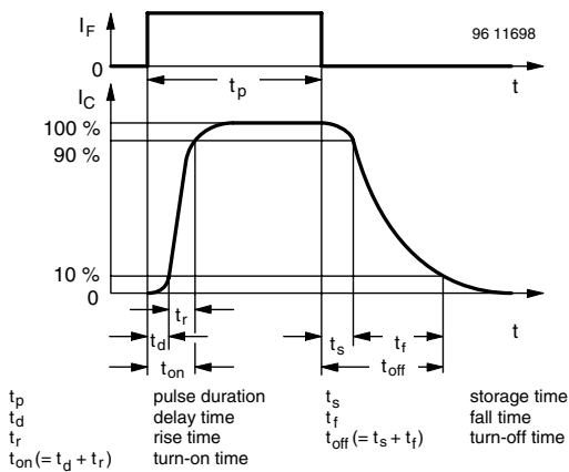
Figure 3. Switching Times
