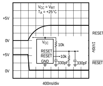
MAX707 RESET, RESET ASSERTION
