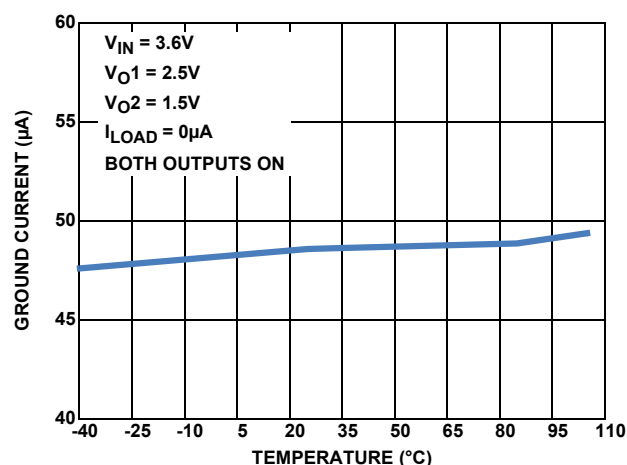
FIGURE 10. GROUND CURRENT vs TEMPERATURE
