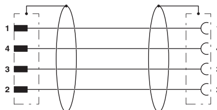
Contact assignment of M12 plugs / M8 sockets
