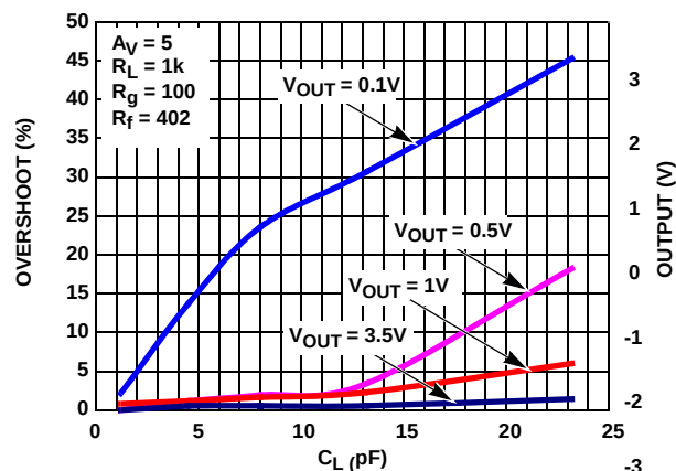
FIGURE 22. ISL55290 PERCENT OVERSHOOT vs V_{OUT} , C_L
