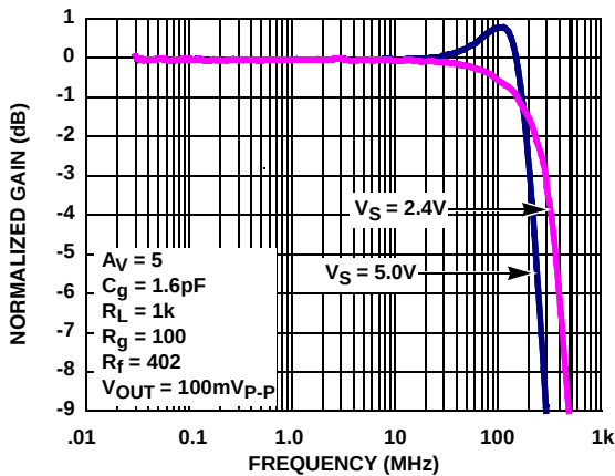
FIGURE 5. GAIN vs FREQUENCY vs V_S
