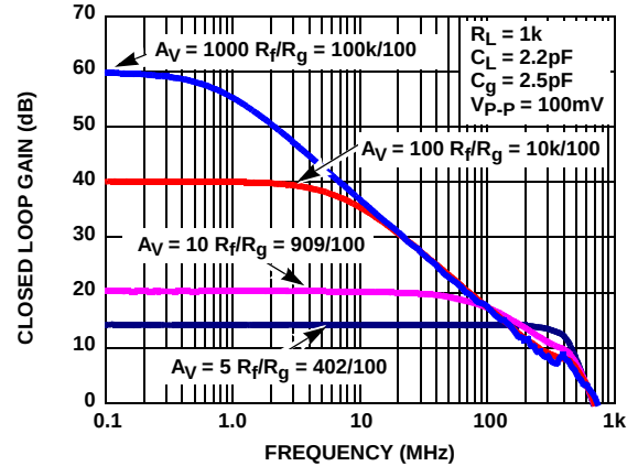
FIGURE 4. CLOSED LOOP GAIN vs FREQUENCY
