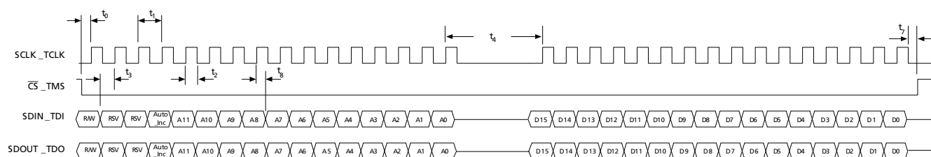
Figure 4-37: Write Mode
