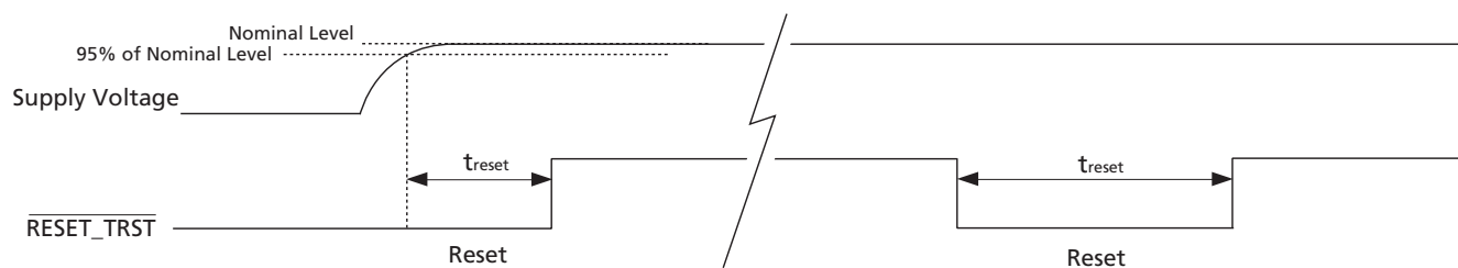
Figure 4-42: Reset Pulse
