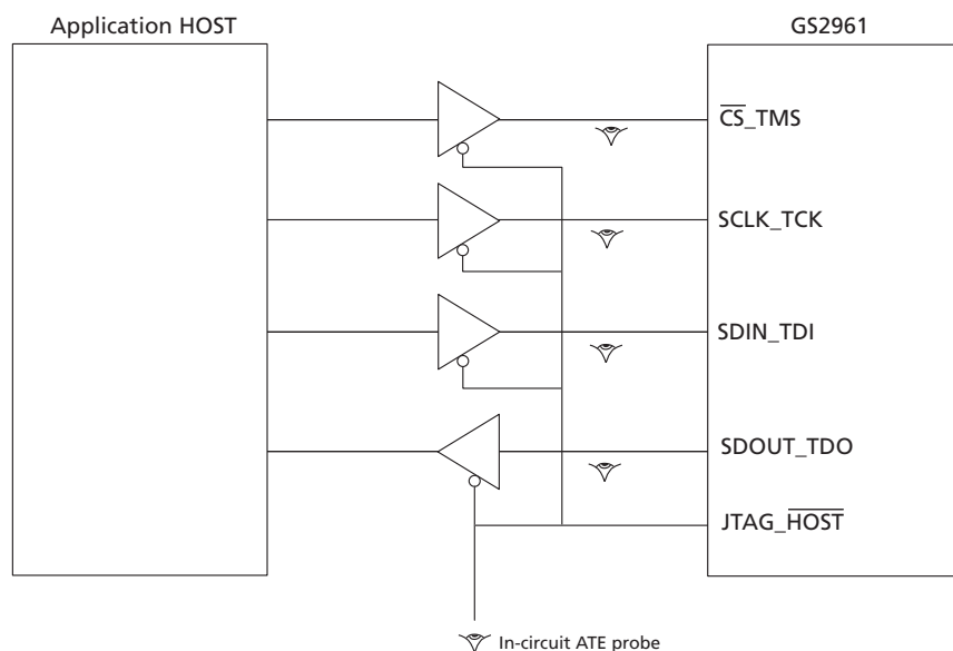
Figure 4-40: In-Circuit JTAG
